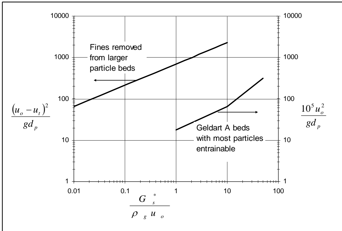
Figure 6-6. Data taken from Kunii & Levenspeil, Fluidization Engineering, 2ed, Butterworth, Boston, 1991 (figure 6 page 175). From this plot the value of G_s^* may be determined for Geldart A particles and for fines removed from larger particle beds.
